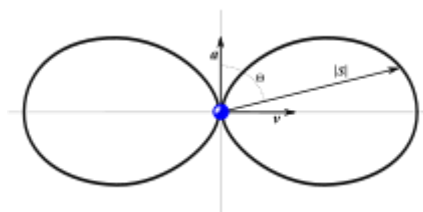
Fig. 1. - The radiation pattern of the dipole emitter in polar coordinates
